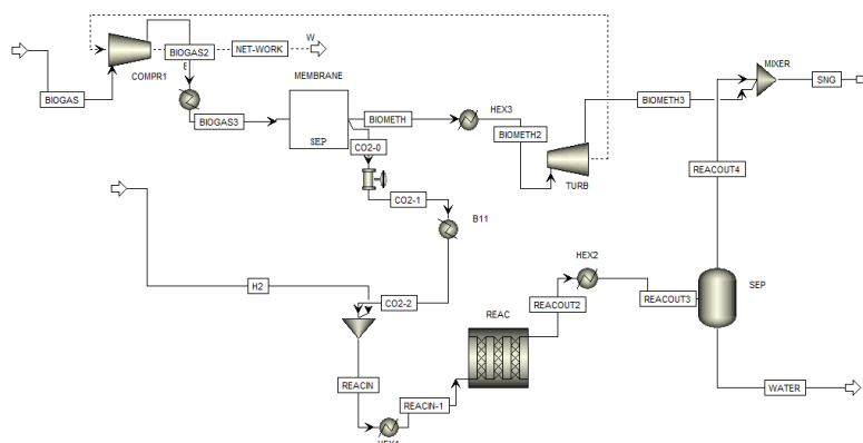
Figure 1: Process flow diagram #1 (PFD-1)
