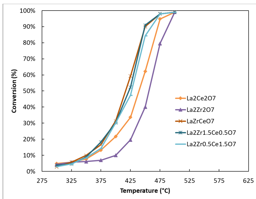
Figure 1: Catalysts screening ( P = 1 atm, T = 300 - 500 °C, Ammonia Feed y_{\text{NH}_3} = 25\% , 60,000 \text{ NmL}^3 \text{ g}^{-1} \text{ h}^{-1} , 200 mg catalyst – 400 mg Qz)
