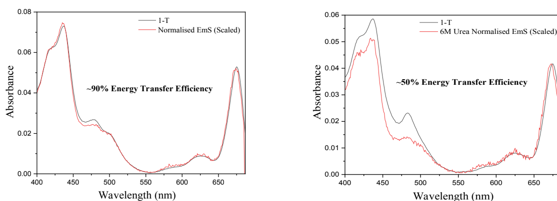
Fig 1. & 2. Excitation-fluorescence-Fluorescence excitation spectra of VCP detected with a fixed emission of at 690 nm for control (left) & and 6M urea (right), respectively.
