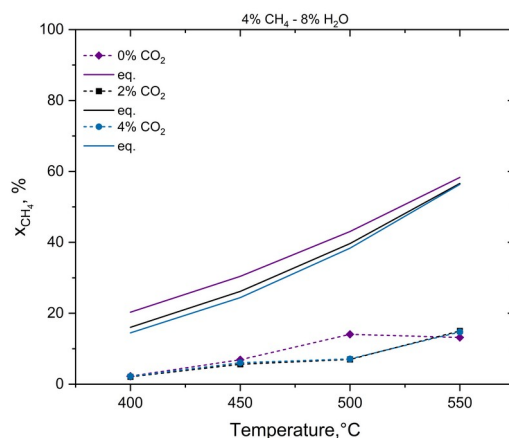
Figure 2: Effect of \text{CO}_2 partial pressure in the feed on methane conversion during SMR.
