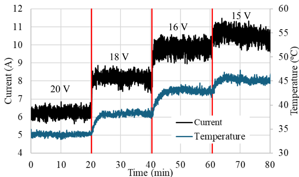
Figure 1: PEMFC current and temperature stability at different operating voltages.
