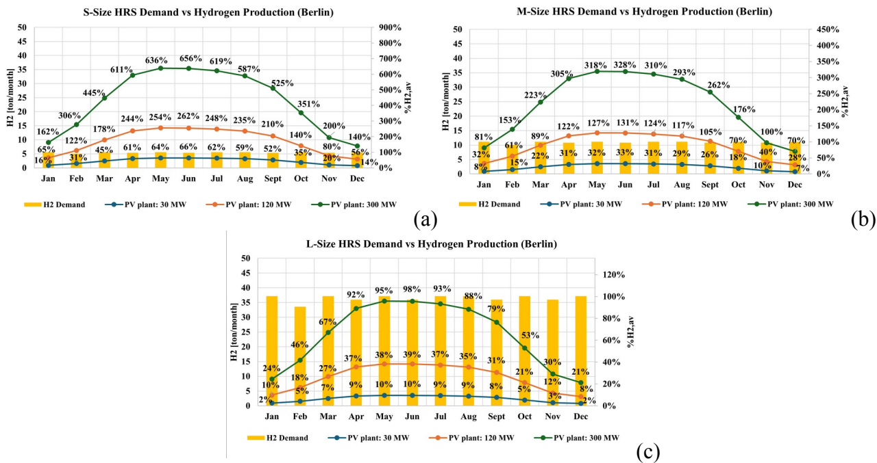
Figure 2. H2 demand vs H2 production in Berlin.
